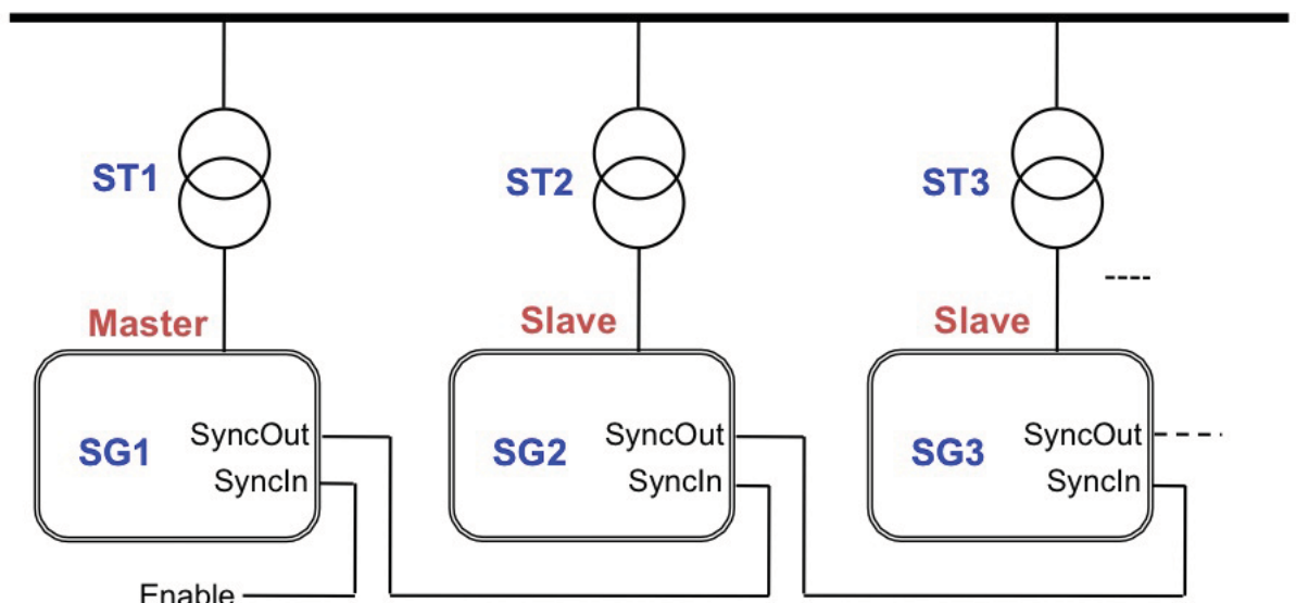
Fig.3 Multiple SGs scenario
