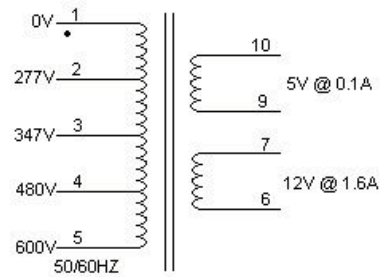
Fig.2 PT configuration
